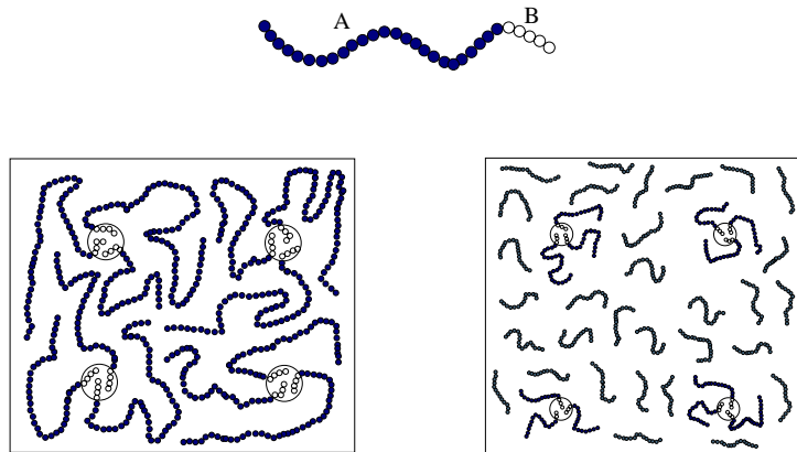
Figure 1: Top: an AB diblock copolymer macromolecule of minority A composition. Bottom: 2D schematic of two possible physical scenarios for the regime considered in this article. Left: microphase separation of very long diblock copolymers with minority A composition. Right: phase separation in a mixture/blend of diblock copolymers and homopolymers of another monomer species having relatively weak interactions with the A and B monomers.
