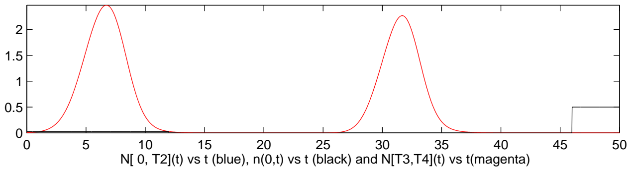
cell density vs age (red) and death rate vs age (black) [Ro, C1, C2, T2] = 20 1 0 12
