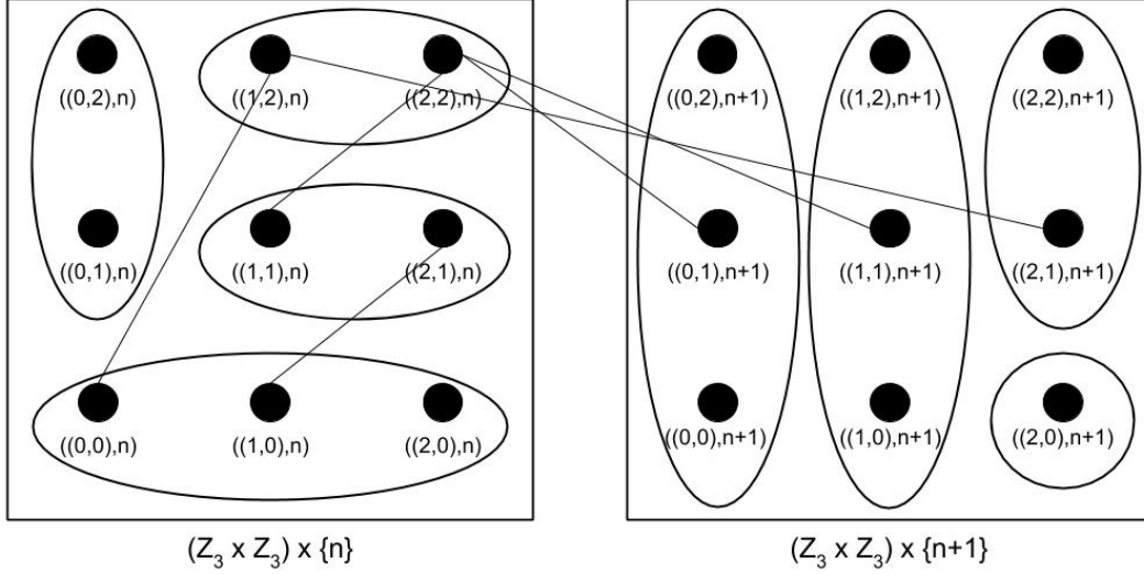
Figure 2: A visual explanation of the proof of Lemma 4 in the case k = 3 . The two squares enclose neighboring (Z_k \times Z_k) -orbits. The circles represent color sets within each orbit. Most edges are omitted, but some are included to show any horizontal color set from the first orbit must admit an edge to every vertical color set from the second orbit. Others are included to show that horizontal color sets in different rows of a single orbit always have edges between them. The same is true for vertical color sets in different columns.
