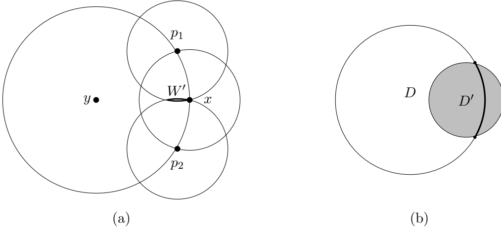
Figure 5.1: (a) The set W' = W'(x, y; r) . (b) When two closed discs intersect, the smaller disc D' contains the shortest arc on the bigger disc D between the intersection points of the boundaries.
