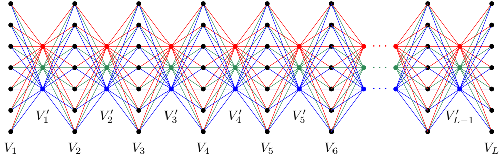
Figure 4: The d -degenerate graph H used in the proof of Theorem 9. In this example, \delta = 7 and d = 3 .
