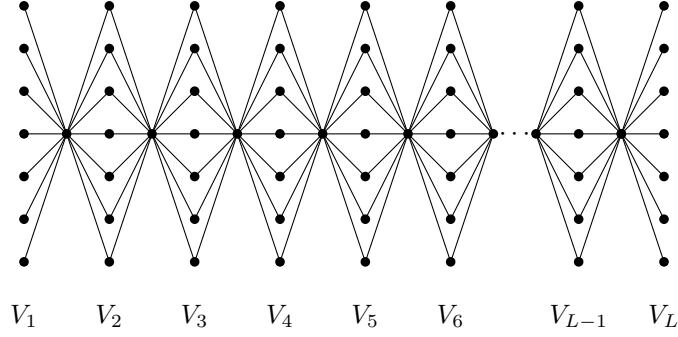
Figure 3: The graph H in the proof of Theorem 8.
