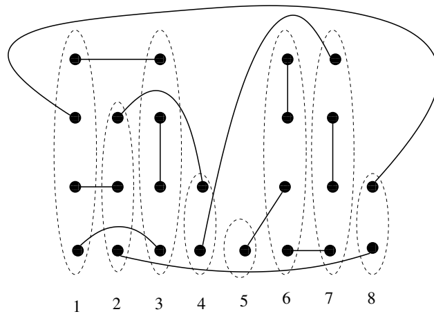
Figure 11.1: Partition of W into cells W_1, \dots, W_8 .
