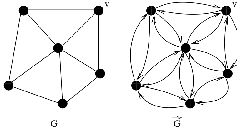
Figure 20.1: Constructing \vec{G} from G .
