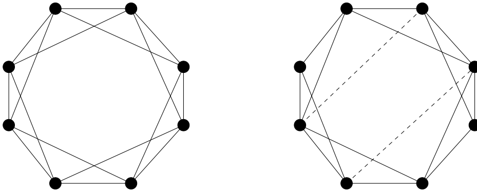
Figure 20.2: C_8 and C_8 after two re-wirings
