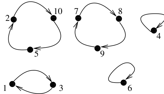
Figure 18.1: A permutation digraph example
