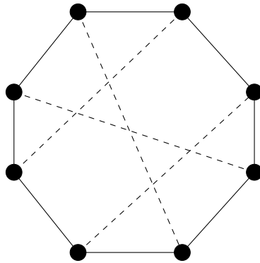
Figure 20.3: C_8 \cup M
