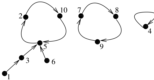
Figure 18.2: A mapping digraph example
