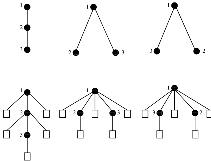
Figure 17.1: Plane-oriented recursive trees and their extensions, n = 3
