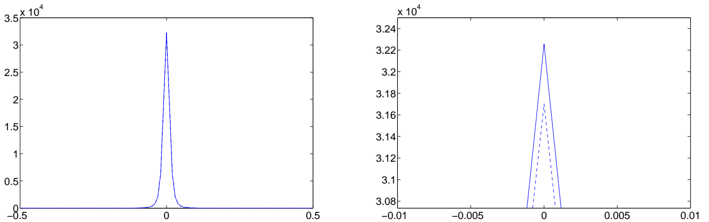
Figure 8.2: contours along the line \mathcal{L} of the density \rho on 101 \times 101 grid using quadratic polynomial approximation p = 2 at later time t = 2 \times 10^{-5} (left column) and zoom view of the same contours (right column). Forward Euler - dashed line, Runge - Kutta - solid line.
