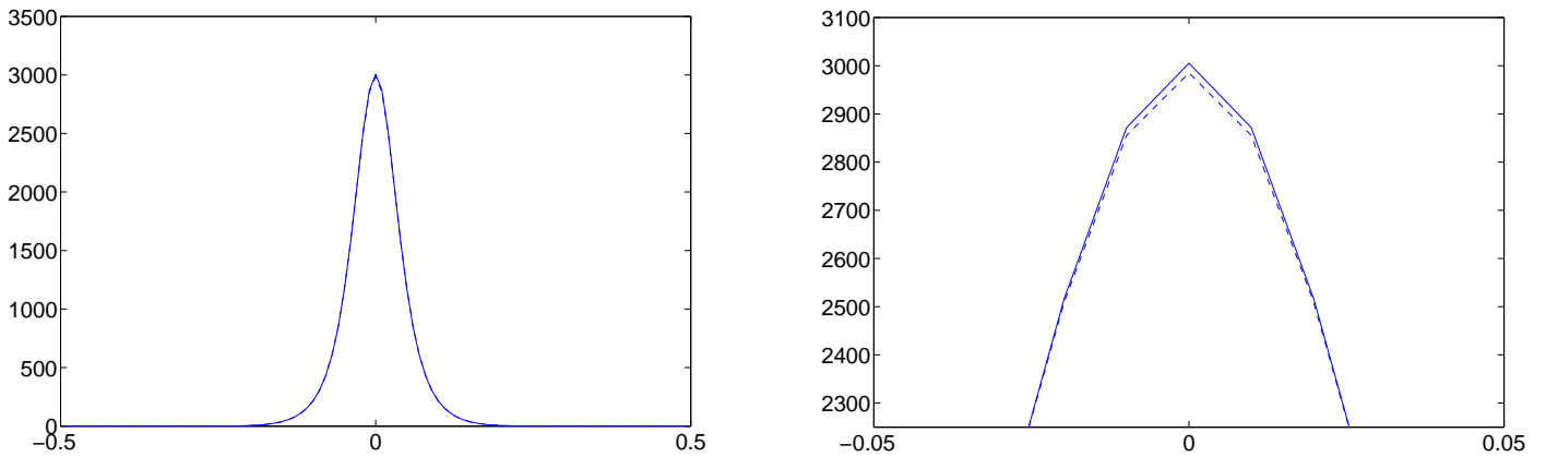
Figure 8.3: contours along the line \mathcal{L} of the density \rho on 101 \times 101 grid using cubic polynomial approximation p = 3 at time t = 5 \times 10^{-6} (left column) and zoom view of the same contours(right column). Forward Euler - dashed line, Runge - Kutta - solid line.
