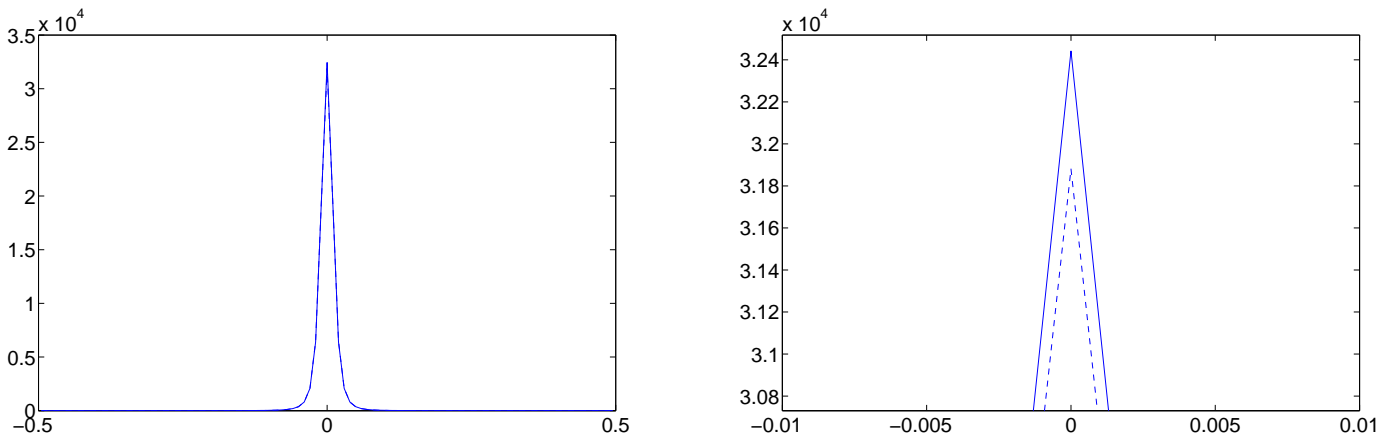
Figure 8.4: contours along the line \mathcal{L} of the density \rho on 101 \times 101 grid using cubic polynomial approximation p = 3 at later time t = 2 \times 10^{-5} (left column) and zoom view of the same contours(right column). Forward Euler - dashed line, Runge - Kutta - solid line.
