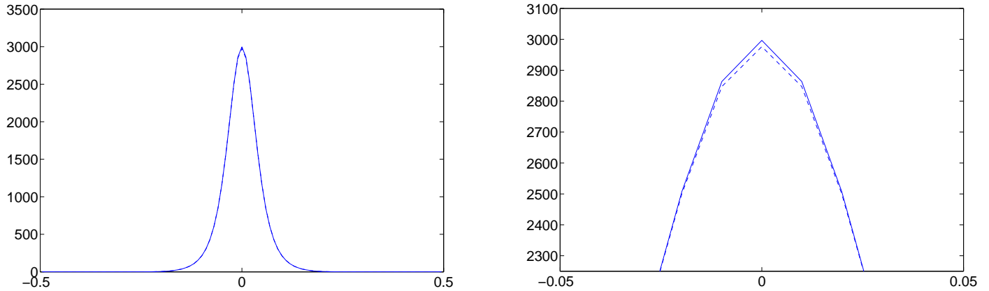
Figure 8.1: contours along the line \mathcal{L} of the density \rho on 101 \times 101 grid using quadratic polynomial approximation p = 2 at time t = 5 \times 10^{-6} (left column) and zoom view of the same contours (right column). Forward Euler - dashed line, Runge - Kutta - solid line.
